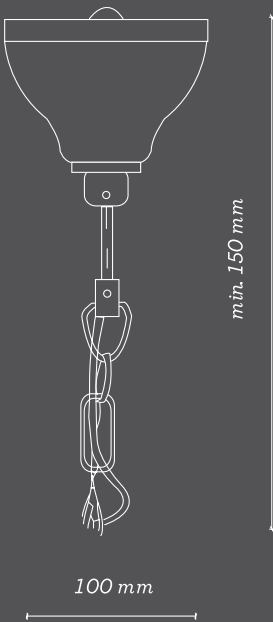
ceiling fixation + cover and adjustable chain
